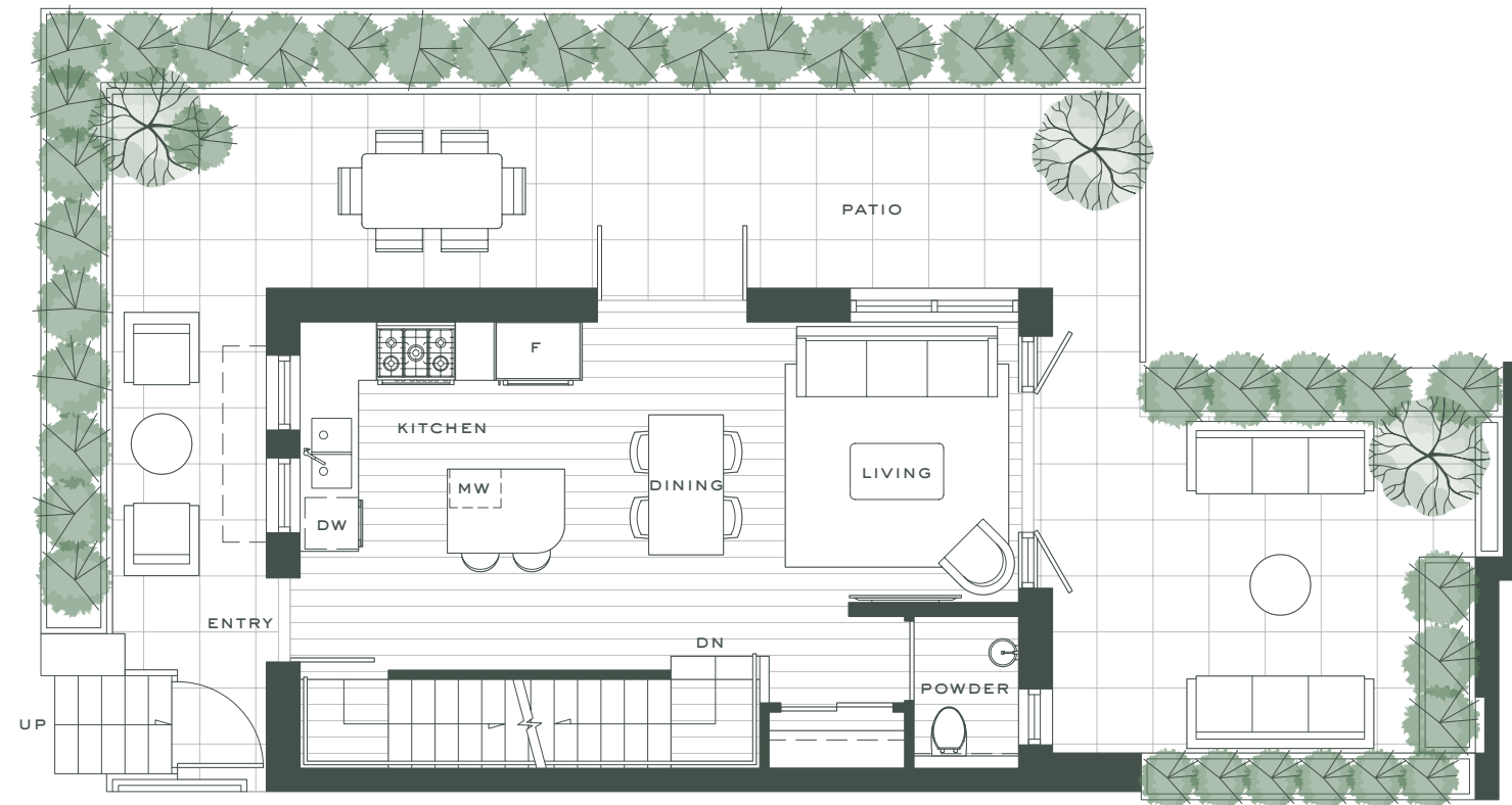
Main
