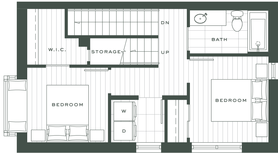
Upper - Level 2
